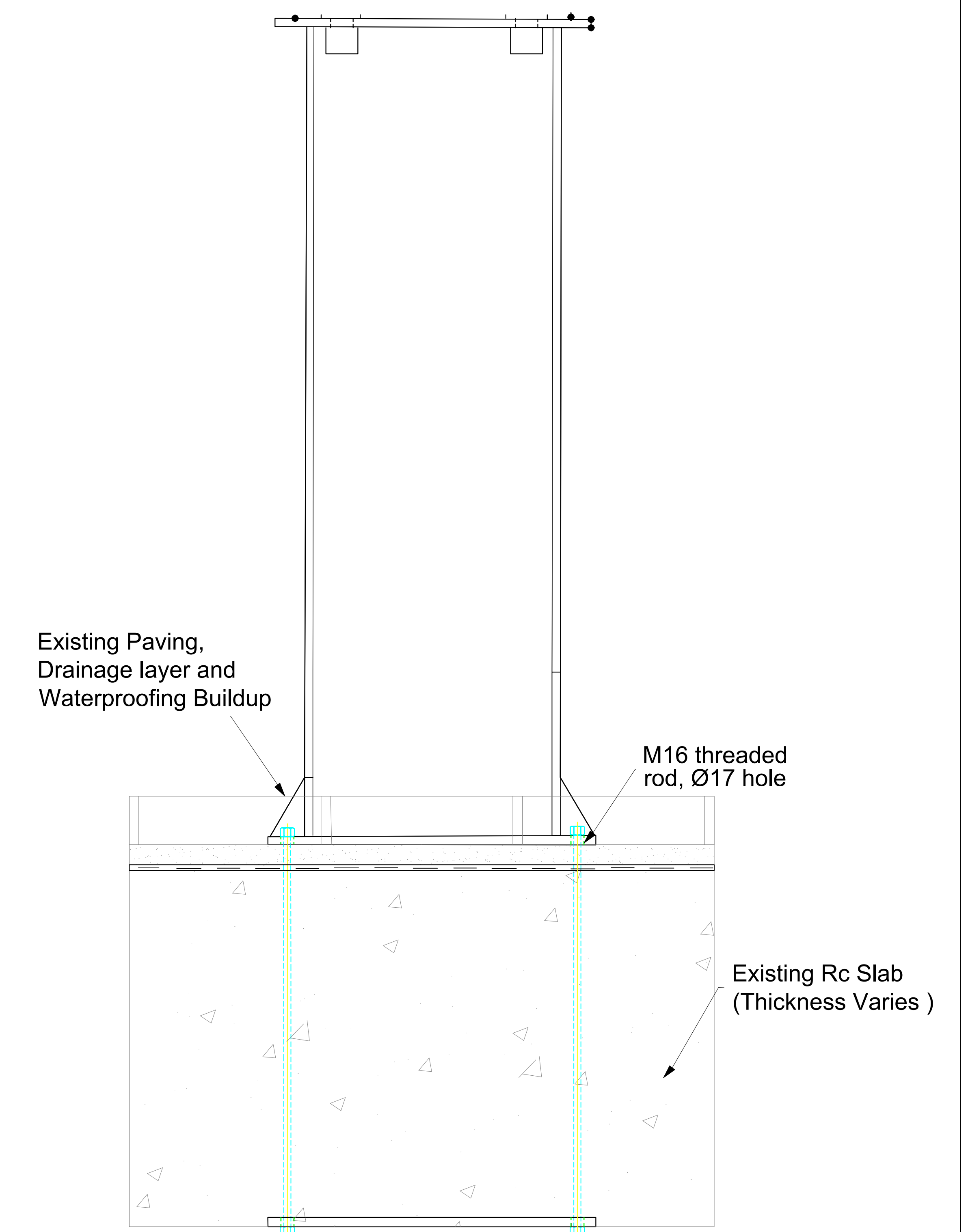
Side View
