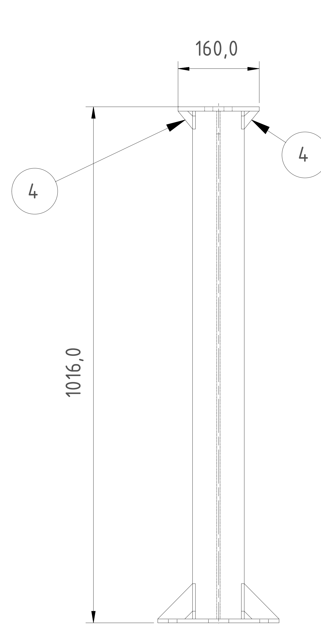
SIDE VIEW ( 1 : 15 )
