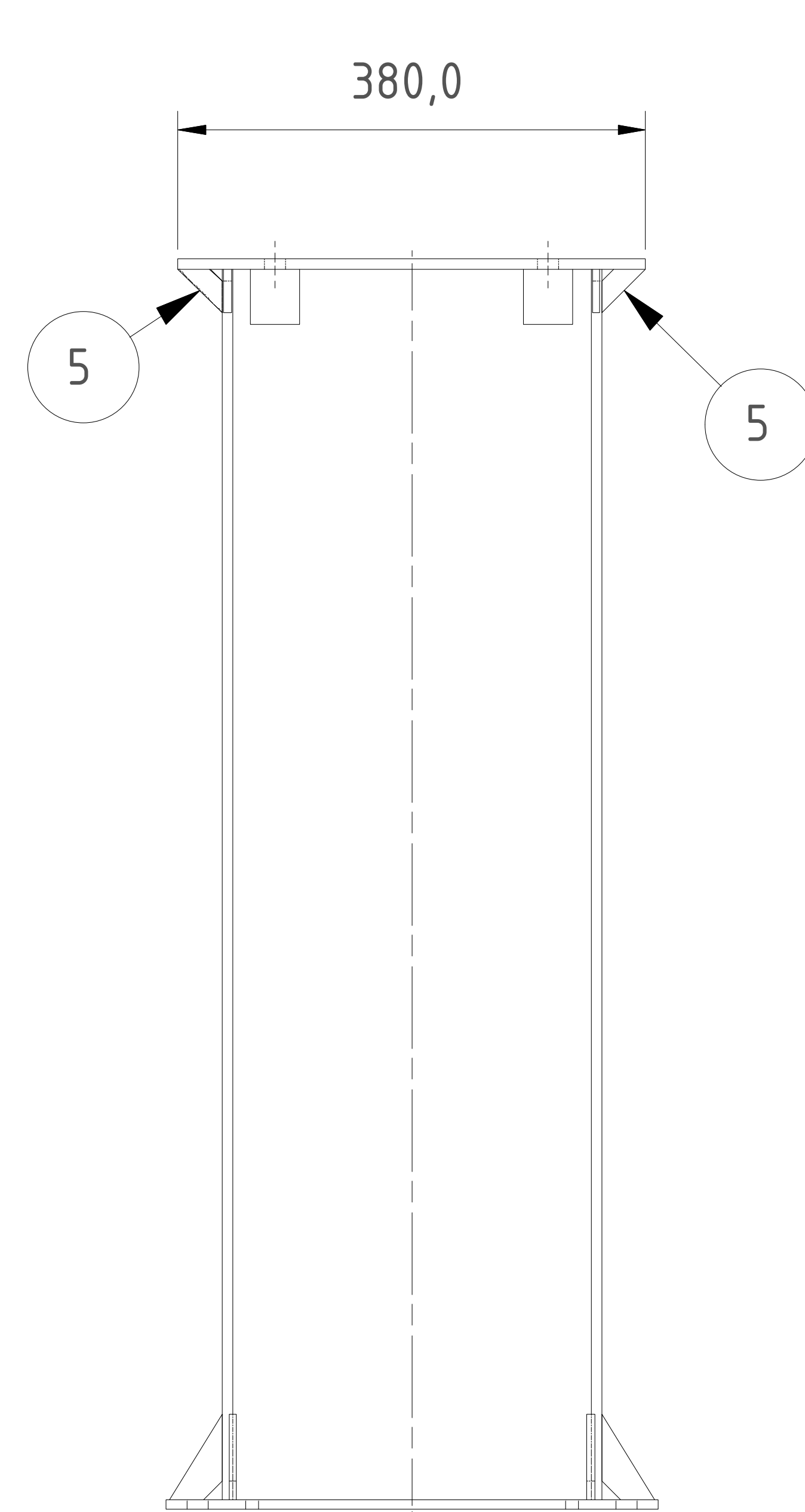
FRONT VIEW ( 1 : 15 )
