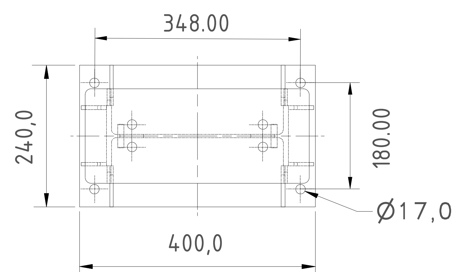
TOP VIEW ( 1 : 15 )
